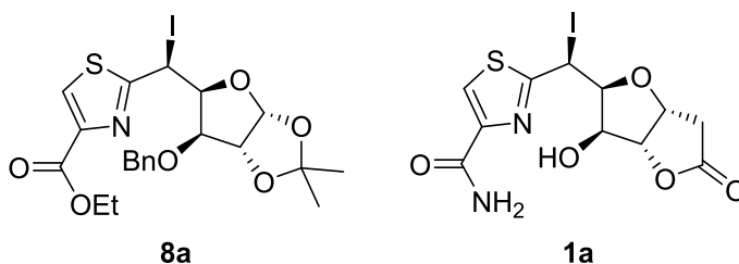
Scheme 1. Obtained ( 8a ) and target ( 1a ) compound
