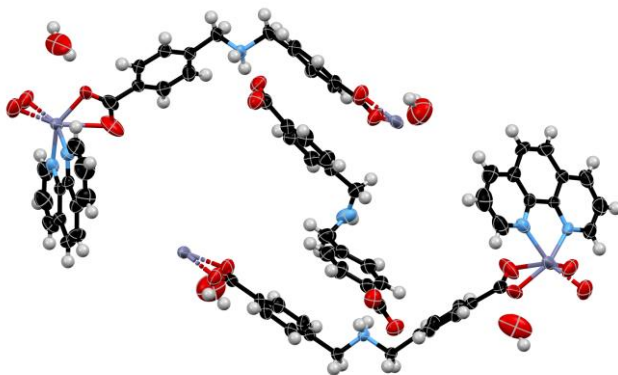
Figure 1. Polymeric structure of complex.
