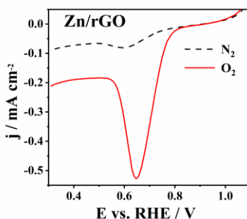
Figure 1. Cathodic scan of cyclic voltammogram of Zn/rGO at 5 mV s -1 in O 2 -saturated 1 M KOH
