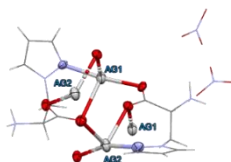
Figure 1. The coordination environment in \{[Ag(\mu-L)]NO_3\}_n .
