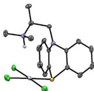
Figure 1. Crystal structure of [PtCl 3 (pmzH)] complex.
