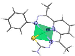
Figure 1. The molecular structure and coordination plane of [\text{Ni}(\text{L}-2\text{H})]
