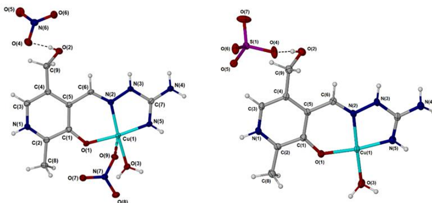
Figure 1. Molecular diagram of [\text{Cu}(\text{PLAG})(\text{NO}_3)(\text{H}_2\text{O})]\text{NO}_3 (left) and [\text{Cu}(\text{PLAG})(\text{H}_2\text{O})]\text{SO}_4 (right) (PLAG = \text{C}_5\text{H}_{13}\text{N}_5\text{O}_2 ) with non-hydrogen atoms represented by 50% displacement ellipsoids and hydrogen atoms as spheres of arbitrary size.
